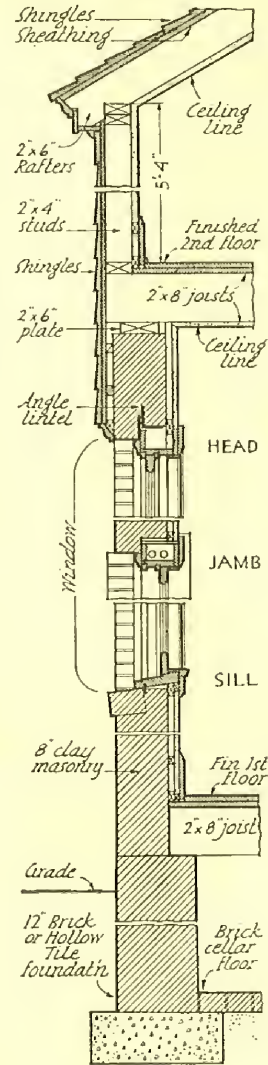
Wall Section
